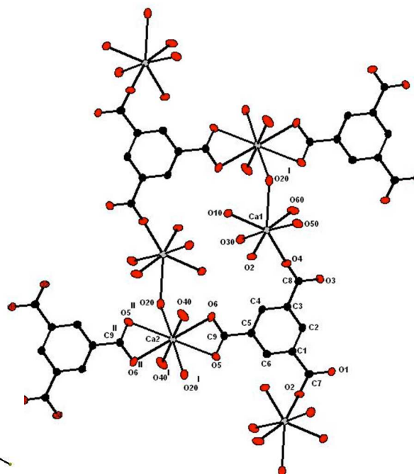
Figure 1. Extended asymmetric unit of [\text{Ca}_3(\text{btc})_2(\text{H}_2\text{O})_{12}]_n . Indexed atoms are obtained by one the following operations : I (1/2 - x, 1/2 - y, 1 - z) ; II (x, 2 - y, 1/2 - z) .
